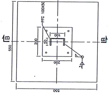
CONCRETE BLOCK DETAIL
