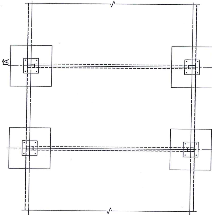
TYPICAL STRUCTURAL FRAMING PLAN TO ACCOMMODATE SINGLE SOLAR PANEL
