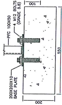
SECTION B-B
